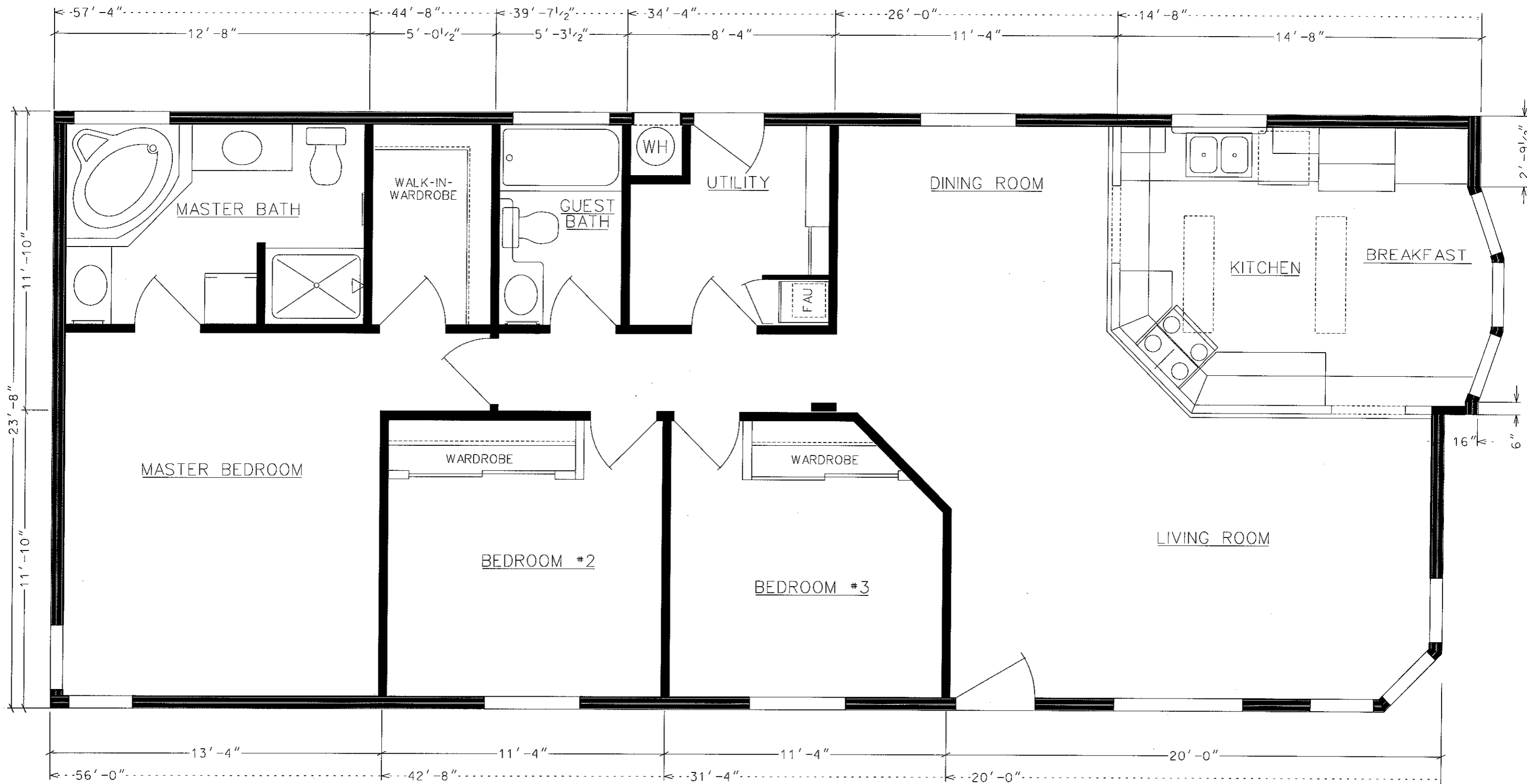
PLAN 24-1939 APPROX. 1,341 SQ.FT 3 BED, 2 BATH 23'-8"X57'-4"/56'-0"
